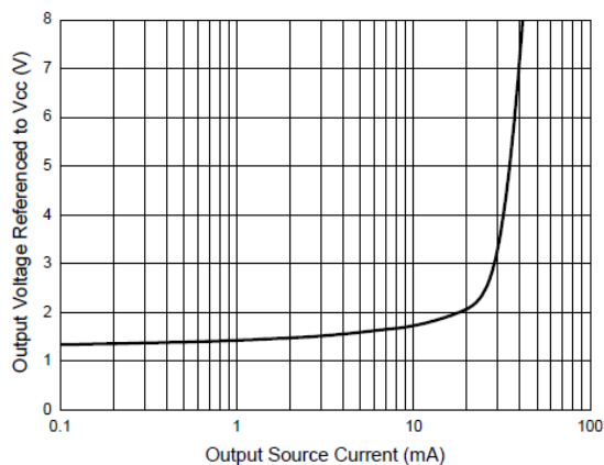
Current Limiting
